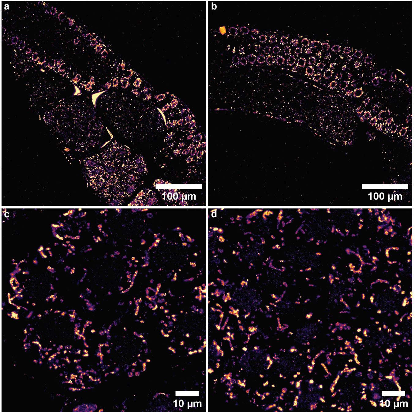
Figure 1. Expansion microscopy of C. elegans with mitochondrial labeling.
